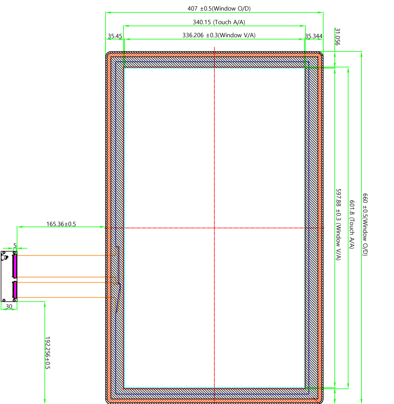
- TOP VIEW (Touch Module) -
