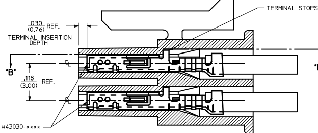
SECTION 'A'-A' WITH TERMINAL (SCALE 10:1)
