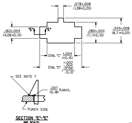
RECOMMENDED PANEL CUT-OUT (SEE NOTES 7 & 9)
