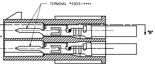
SECTION 'D'-D' WITH TERMINAL SCALE B)
