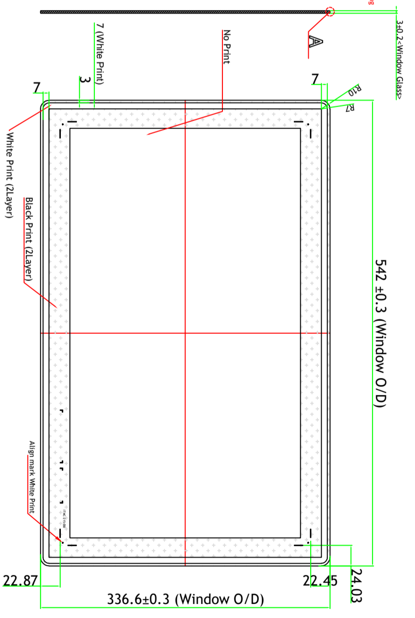
Rear View
