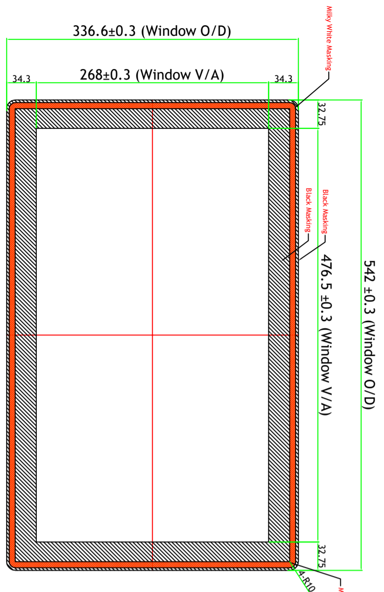
Front View
