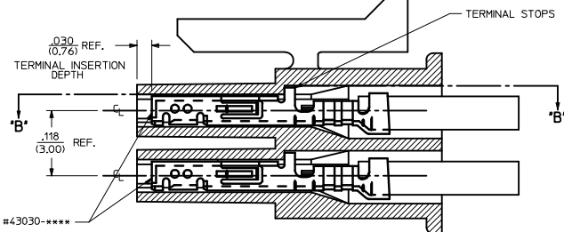
SECTION 'A'-A' WITH TERMINAL (SCALE 10:1)
