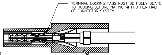
SECTION 'B'-B' (SCALE 10:1)
