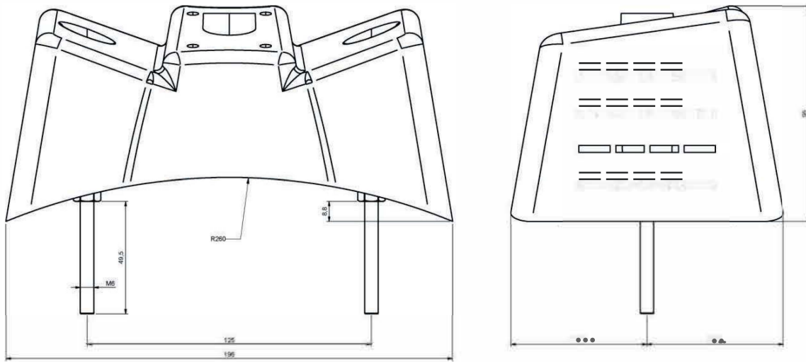
Figure 15: Base Topper R260 curved (104-0015-2)
