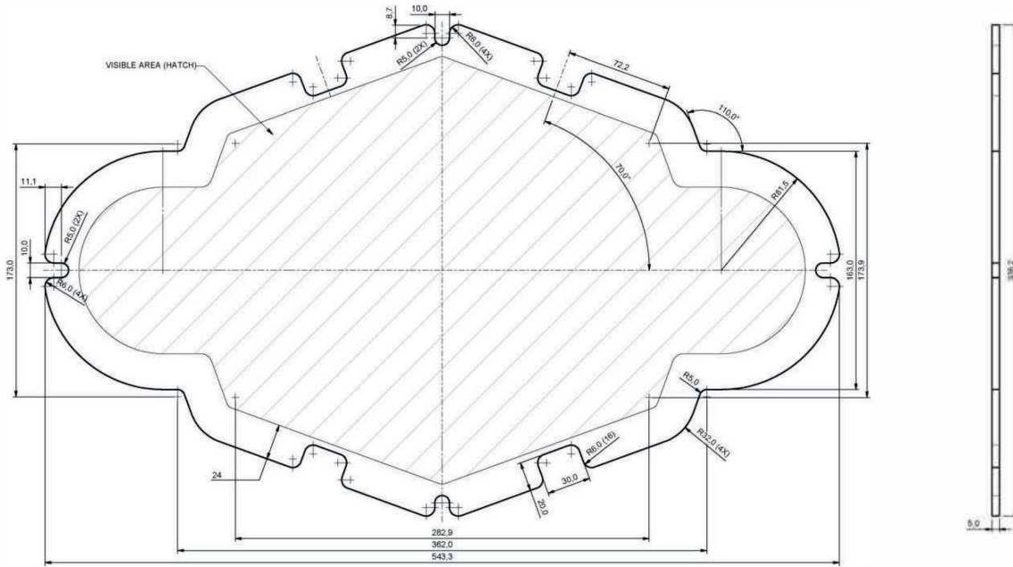
Figure 5: Front plate Ringo Compact (104-0101)
