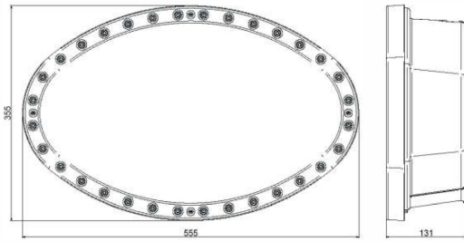
Figure 1: Ellipse Compact model
