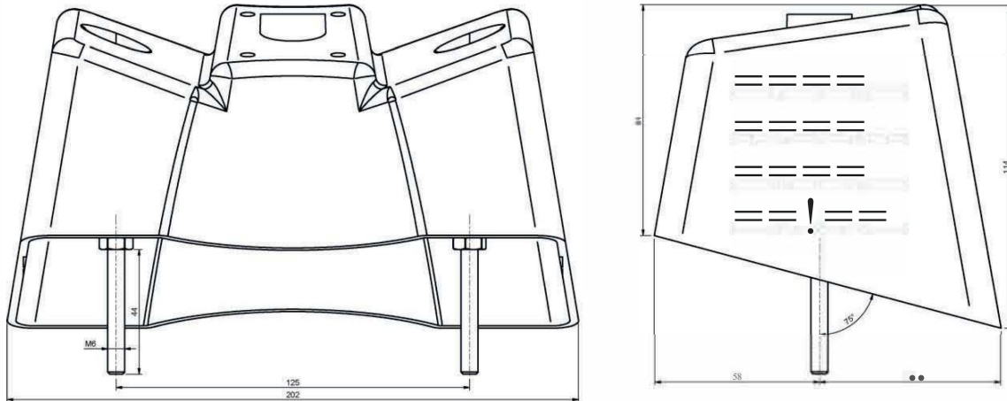
Figure 13: Base Topper 15 Degrees slanting (104-0010-2)
