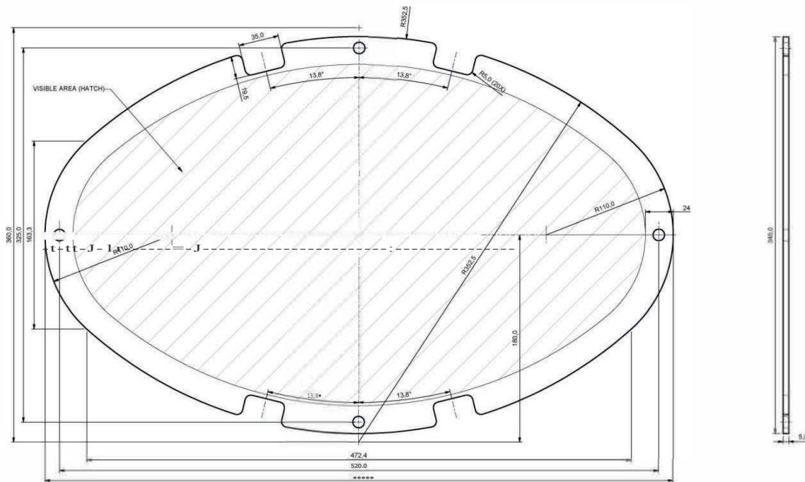
Figure 6: Front plate Elipse Compact (104-0201)
