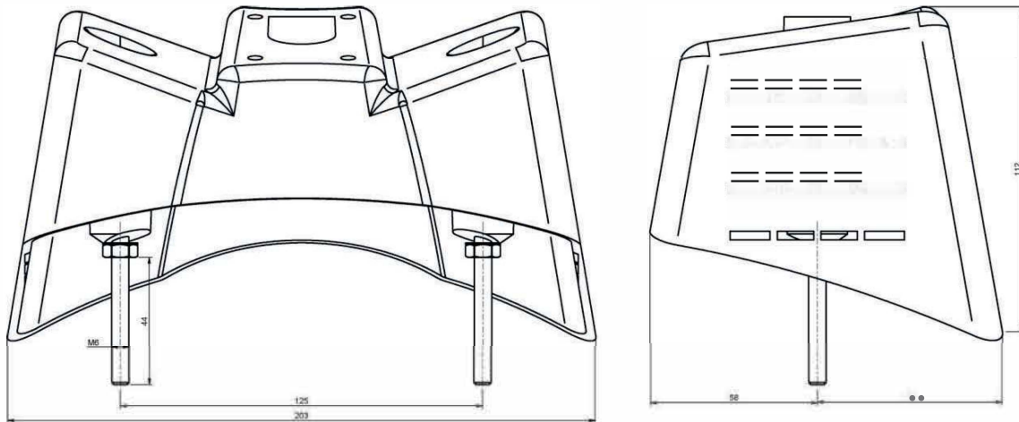
Figure 14: Base Topper R260 curved (104-0014-2)
