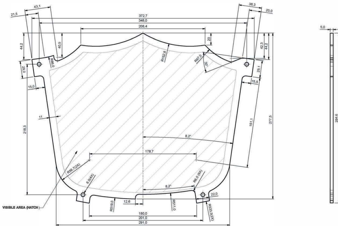
Figure 7: Front plate Shield (104-0301)
