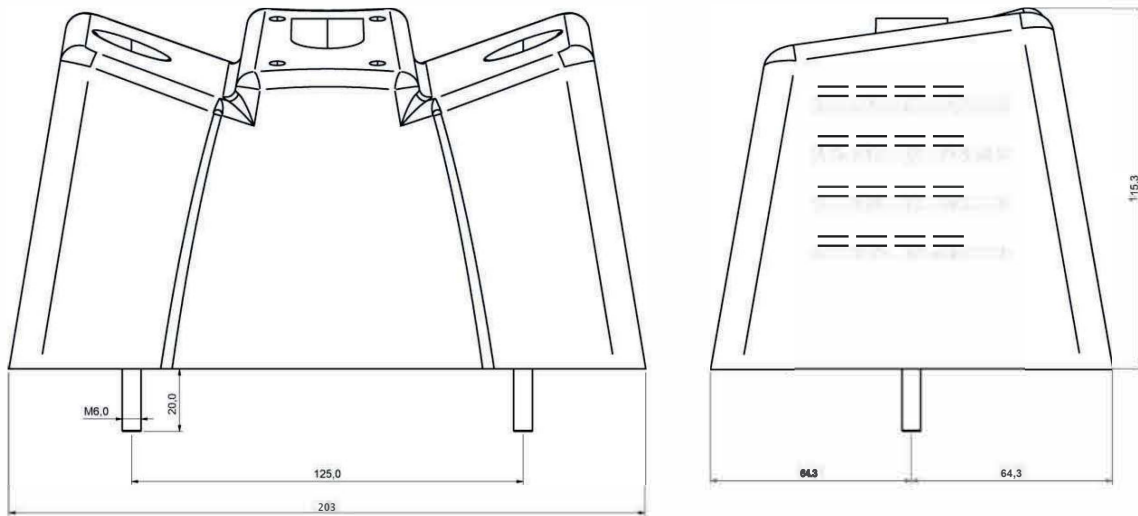
Figure 16: Base Topper flat mounting (104-0020-2)
