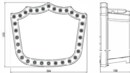
Figure 3: Shield model
