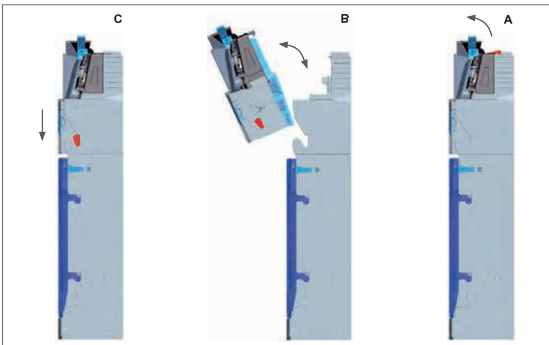
Fig. 4: Removing and reinstalling coin validator
