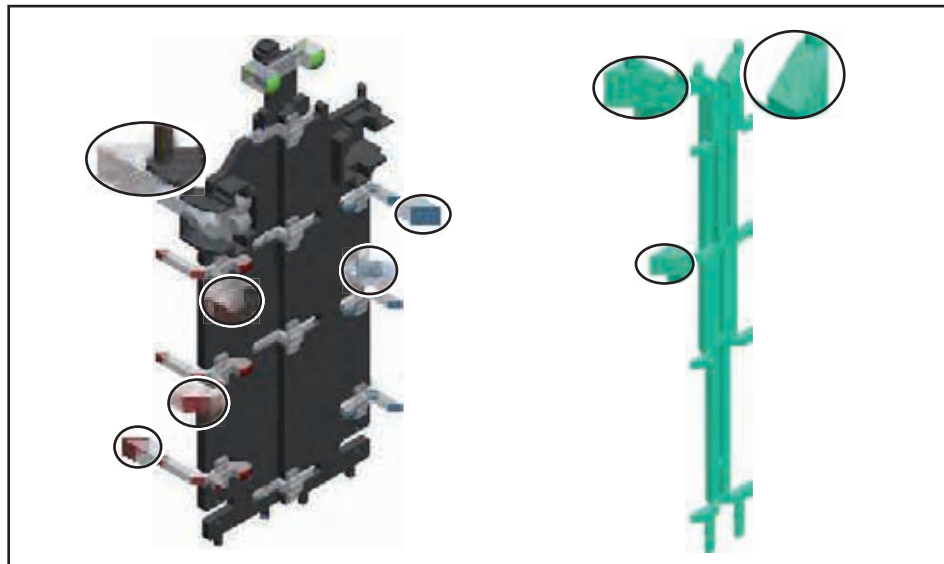
Fig. 16: 45° surfaces of light transmitter and light collectors
