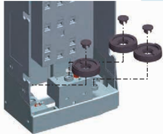
Fig. 8: Removing and reinstalling payout discs and lockings
