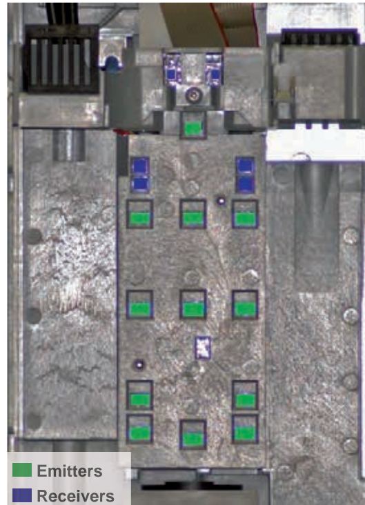
Fig. 14: Housing cut-outs for emitters & receivers on interface module
