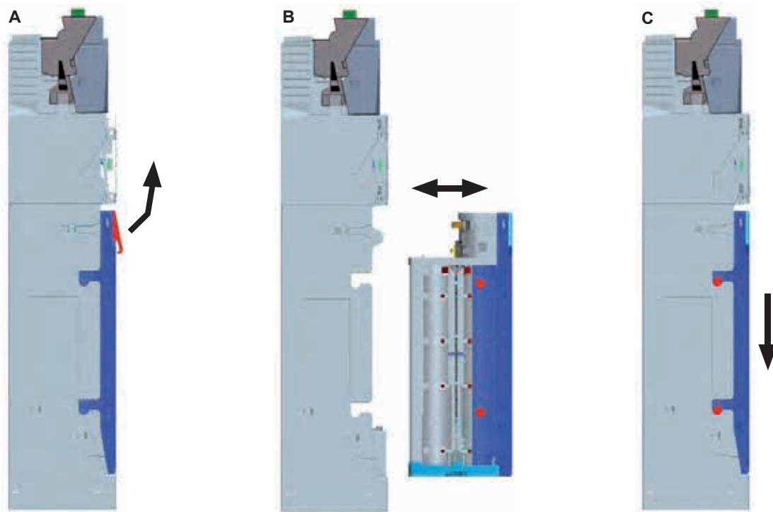
Fig. 7: Removing and reinstalling the coin cassette
