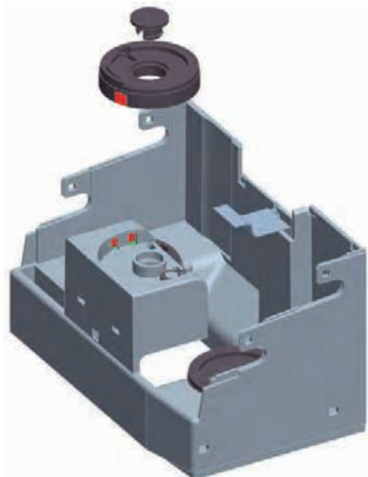
Fig. 10: Sensors on payout disc receptacle
