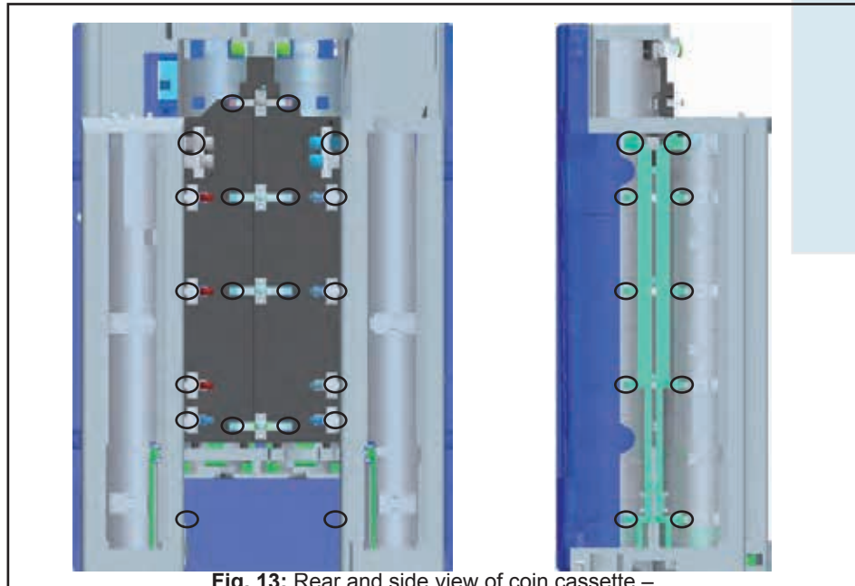
Fig. 13: Rear and side view of coin cassette – all 45° surfaces accessible
