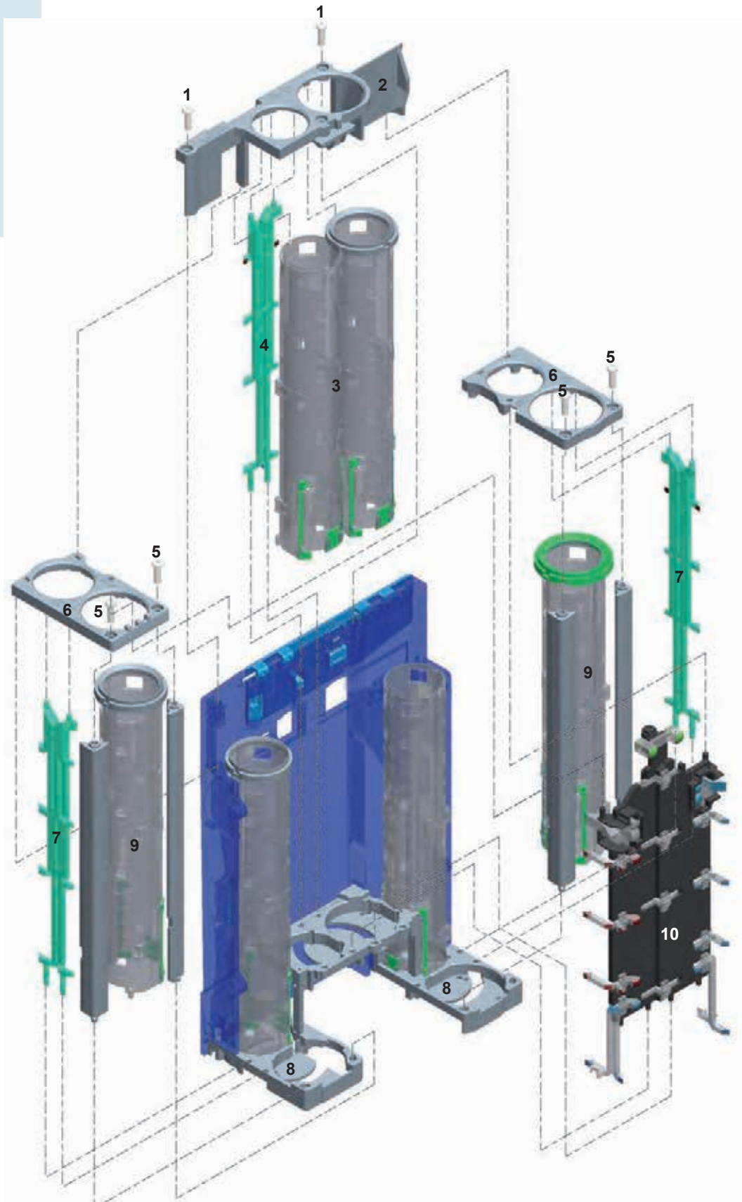
Fig. 15: Assembly plan for coin cassette
